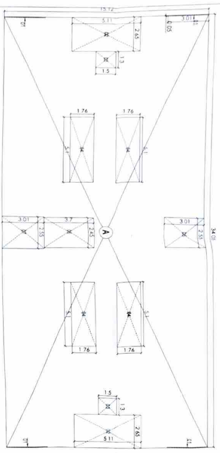
TYPICAL AREA DIAGRAM OF GR., 1ST, 2ND & 3RD FLOOR (SCALE = 1:100)
