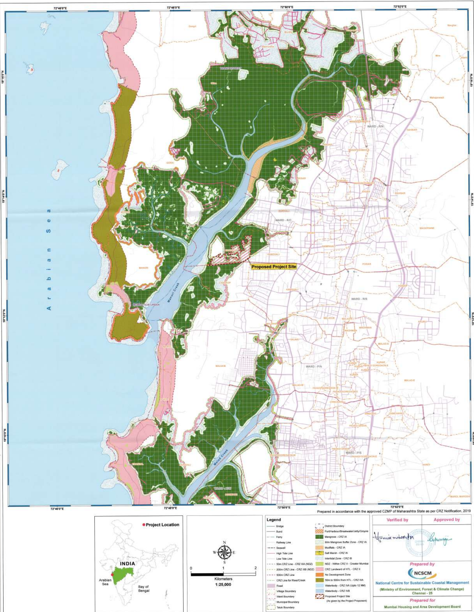
Figure 4: CRZ Map covering about 7 Km around the Proposed Project Site (Refer Report No. NCSCM/CRZ-Cell/CRZ-R04/2024/34)
